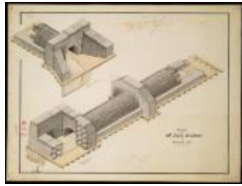
Plan of 6ft. Arch-Culvert on Section 322 (NYSA_B0380-85_0465)
